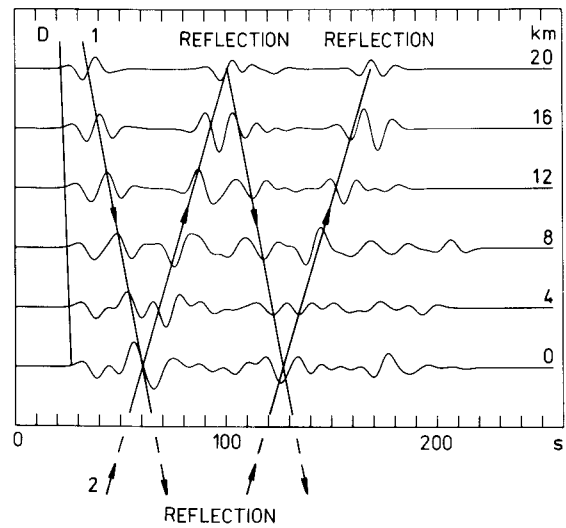
Fig. 7. Synthetic section with marked direct wave denoted by D and local interference waves propagating horizontally from the right ( left ) margin of the basin to the left ( right ) denoted by 1 (2). After reaching the opposite side of the basin, waves 1 and 2 are reflected back
