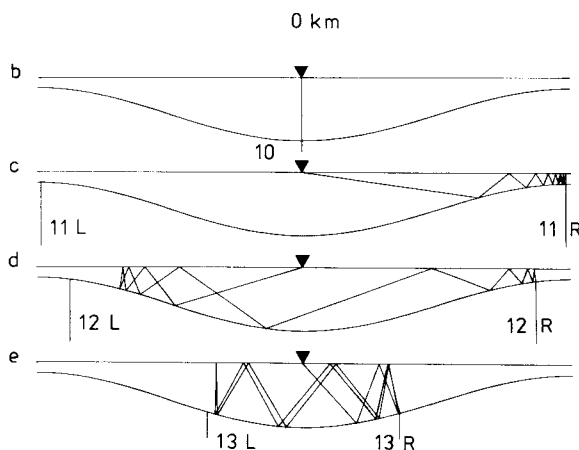
Fig. 6. a Formation of the wave field at the receiver at 0 km. Four branches formed by various waves propagating along various types of rays are denoted by numbers 1-4. b-e Examples of 8-times-reflected rays; the rays incident on the left margin of the basin and denoted by L would have trajectories symmetrical to the rays incident on the right margin of the basin. The rays of type b contribute to line 1 in a ; of type c to 2; d to 3 and e to 4
