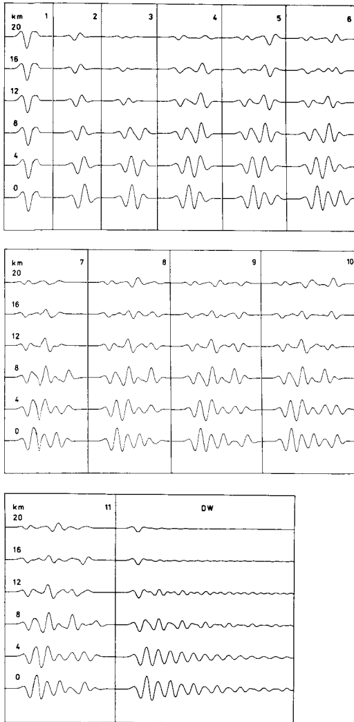
Fig. 8. Comparison of ray and discrete wavenumber synthetics for a prevailing wavelength of approximately 28 km ( T_p = 40 s). The results of the discrete wavenumber method are denoted by DW. The synthetics with numbers are ray synthetics which include successively increasing numbers of multiples: 1 direct wave only, 2 superposition of the direct wave and once-reflected wave etc.
