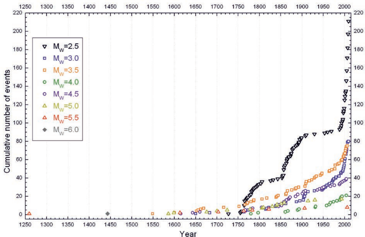
Fig. 6. The cumulative number of events versus time for different magnitude intervals, based on the declustered SLOVEC (2011) catalogue. The increment between the magnitude classes is M_w=0.5 .
