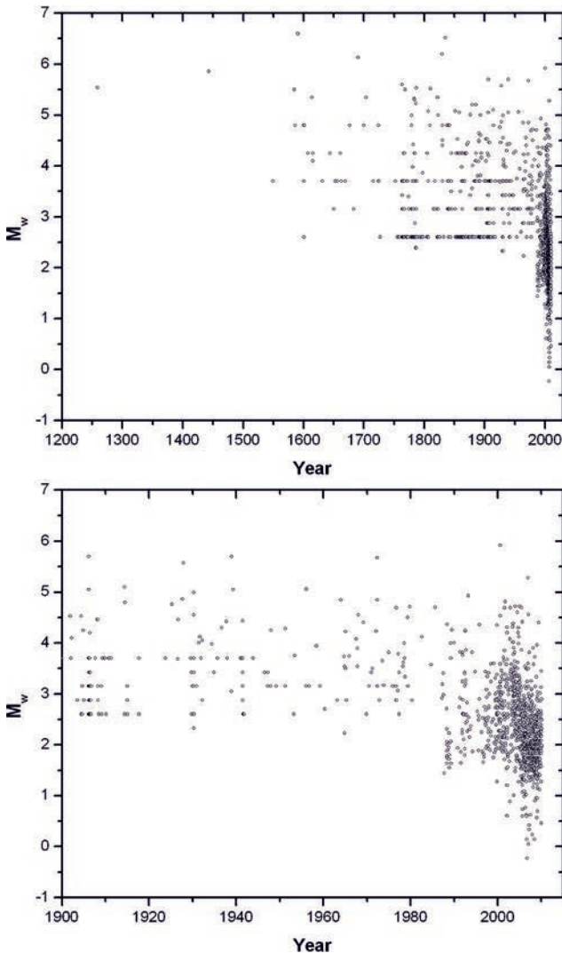
Fig. 7. Time–Magnitude distribution for the unified and homogenized SLOVEC (2011) catalogue.
